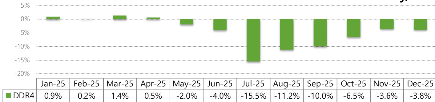
DDR4 Sufficiency, 2025
